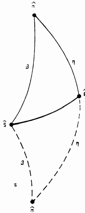
FIG. 1. Spin-Axis Attitude from Two Arc-Length Measurements.
