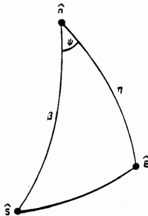
FIG. 2. Spin-Axis Attitude from the Measurement of Two Arc Lengths and One Dihedral Angle.
