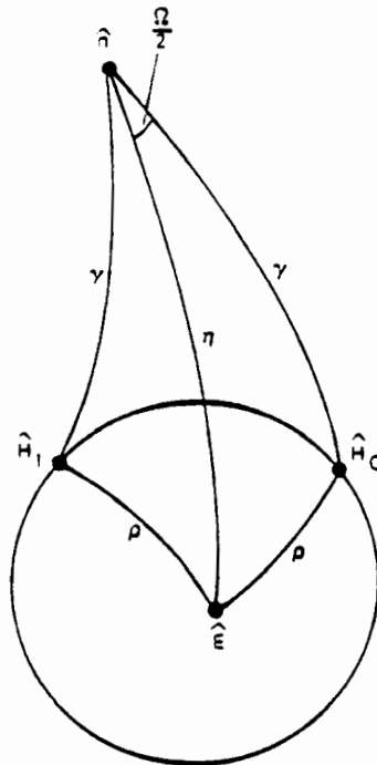
FIG. 3. Geometry of the Nadir-Angle Computation.
